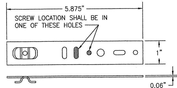
① INSTALLATION CLIP MIN. 50 KSI GALV. STEEL
