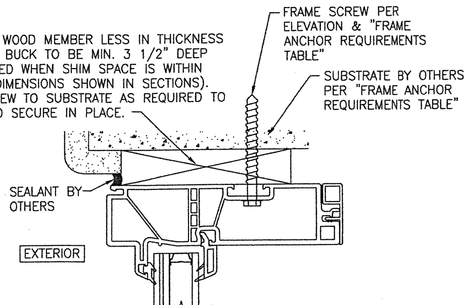
OPTIONAL DIRECT MOUNT DETAIL TO SUBSTRATE WITH SPACER (HEAD SECTION SHOWN; SILL & SIDES ARE INSTALLED THE SAME)
